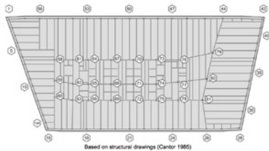
A floor plan of WTC 7. According to NIST, Column 79 on the northeast side was the first column to fail.
