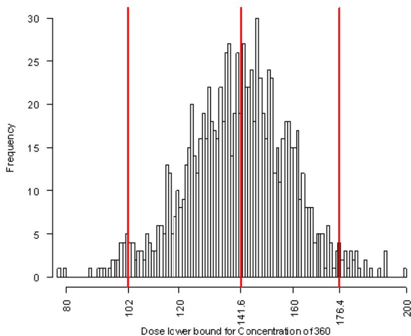
Figure 5. Histogram of aspartame dose lower bound (x-axis in mg/kg bw) considering \alpha = 0.05 for phenylalanine plasma level threshold of 360 µM.
