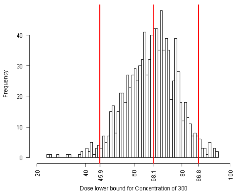
Figure 12. Histogram of aspartame dose lower bound (x-axis in mg/kg bw) considering \alpha = 0.05 for phenylalanine plasma level threshold of 300 µM.
