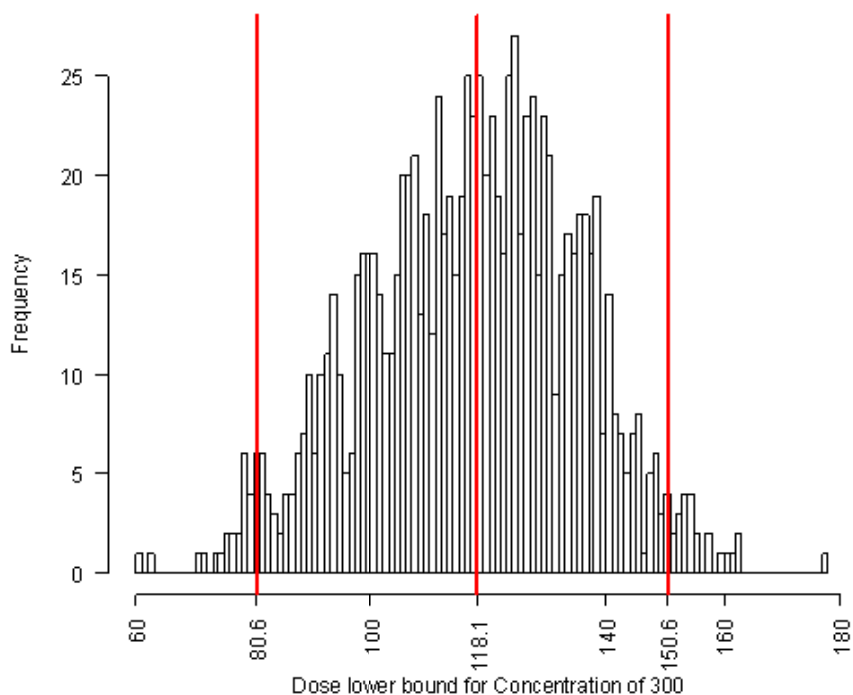
Figure 4. Histogram of aspartame dose lower bound (x-axis in mg/kg bw) considering \alpha = 0.05 for phenylalanine plasma level threshold of 300 µM.
