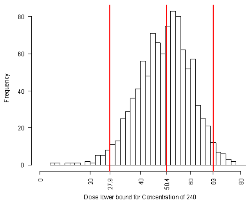
Figure 11. Histogram of aspartame dose lower bound (x-axis in mg/kg bw) considering \alpha = 0.05 for phenylalanine plasma level threshold of 240 µM.
