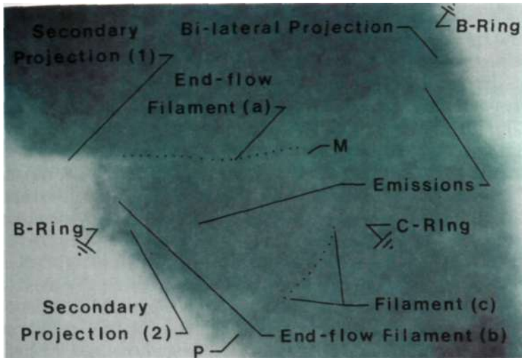
Plate 22: B-ring emissions become C-ring constituents.
