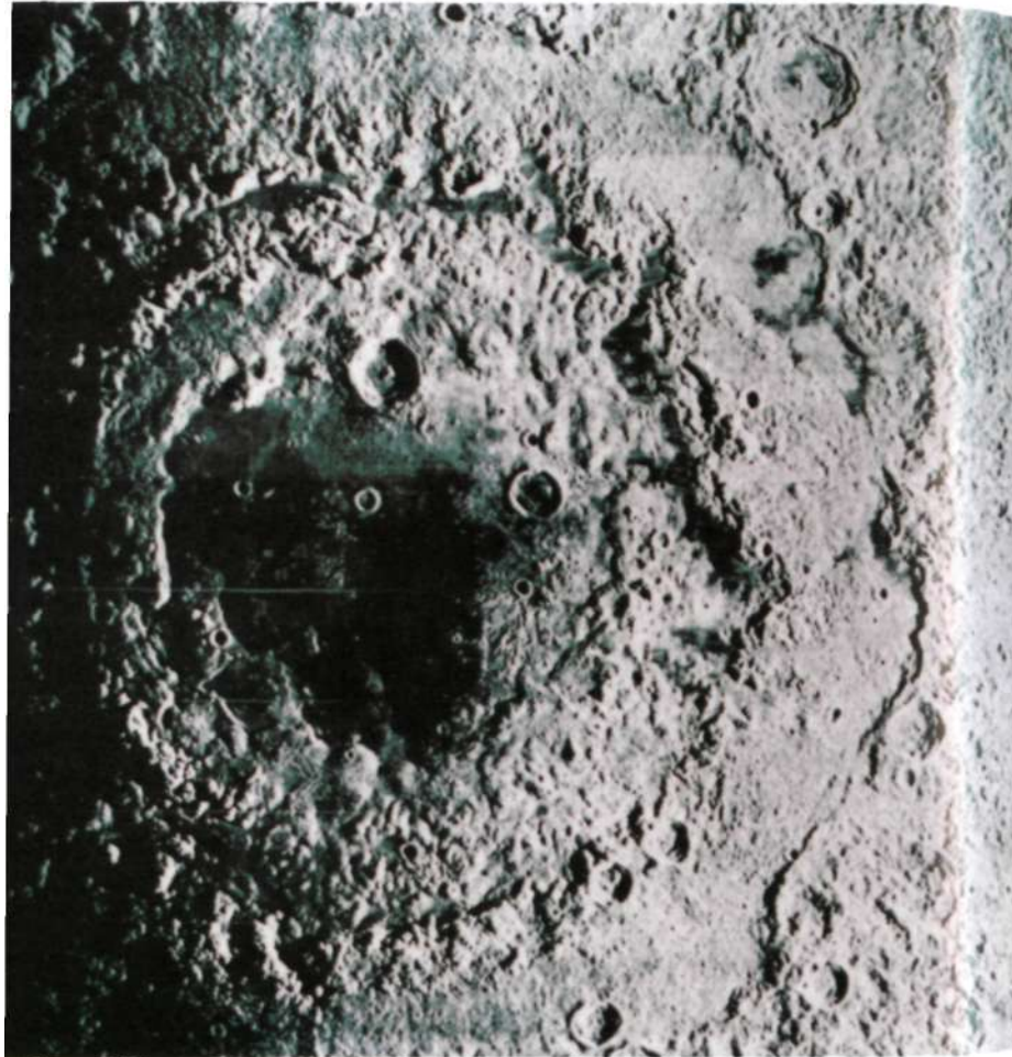
Mare Orientale, anciently imprinted on Earth's moon by an "E.M.V.", remains a demonstrative statement of awesome power. Photograph, which includes only part of the affected area, is a mosaic assembled by NASA from circumlunar flights.
