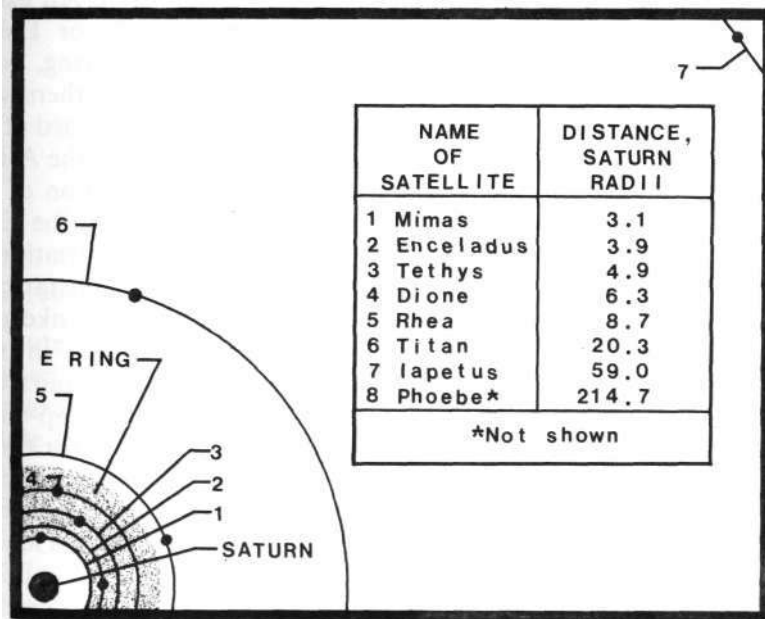
(b) Spherical Satellites
