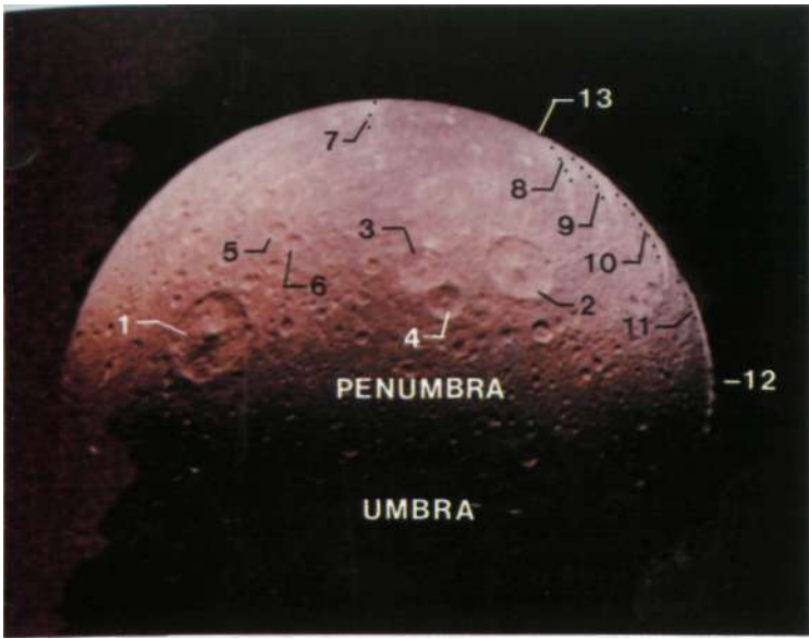
(a) Photographic identifications
