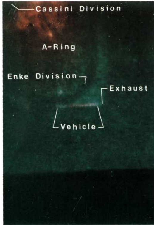
Plate 8: A second vehicle substantiates the process by which the outer A-ring and the Enke division are formed.
