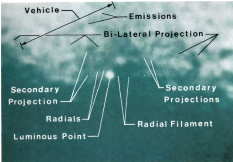
Plate 15: Luminous point of Plate 14 essentially is an arc light whose apparent power source is a remote vehicle capable of generating paths carrying electricity.
