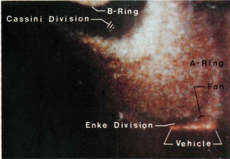
Plate 7: Formation of the Enke division.
