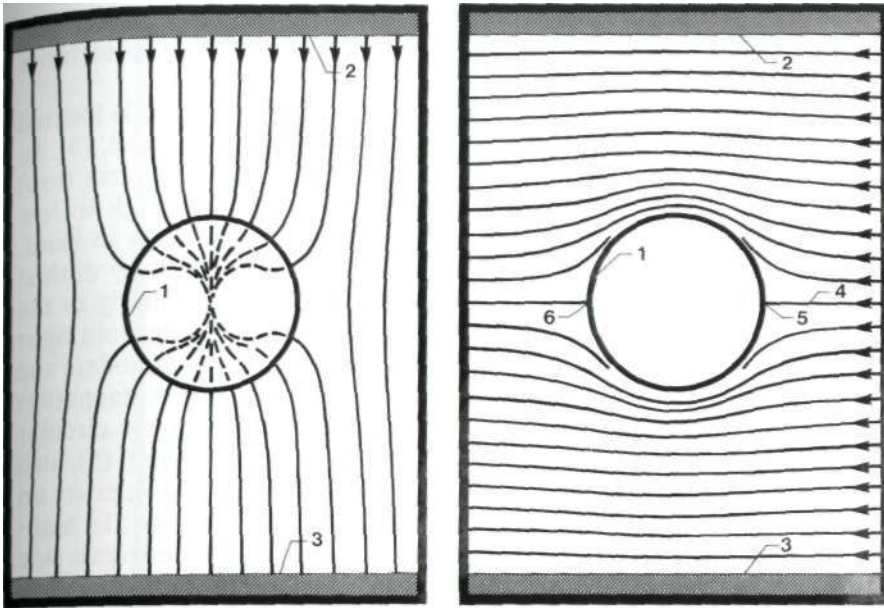
(a) Current paths
