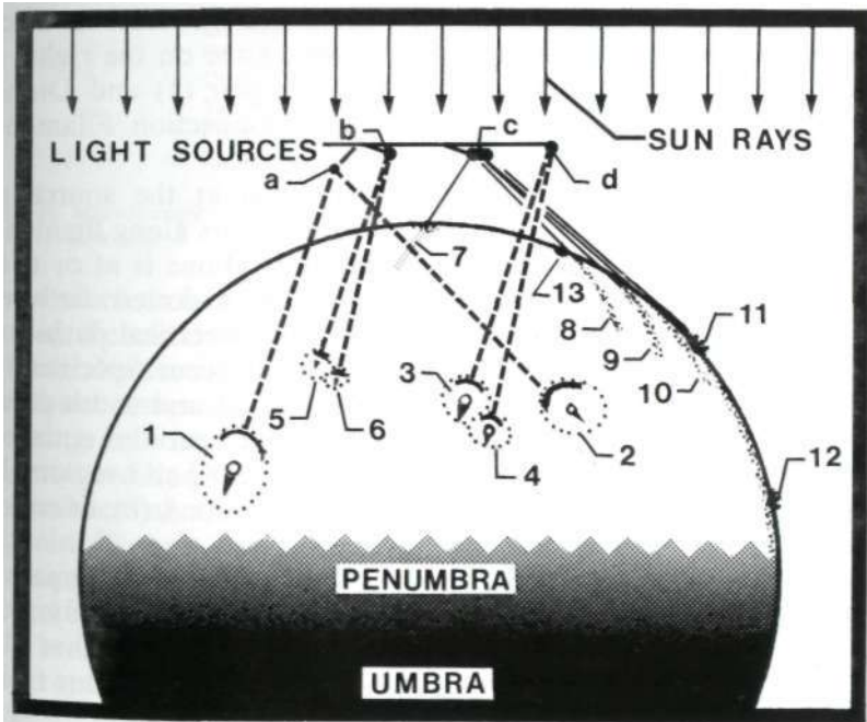
(b) Pictorial interpretation aids
