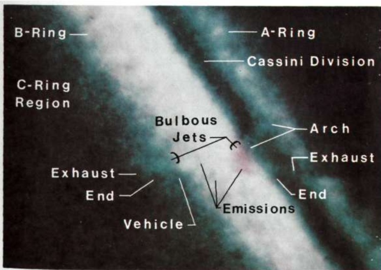
late 9: Partially developed ring system exhibiting a transversely positioned cylindrical vehicle i the B-ring.
