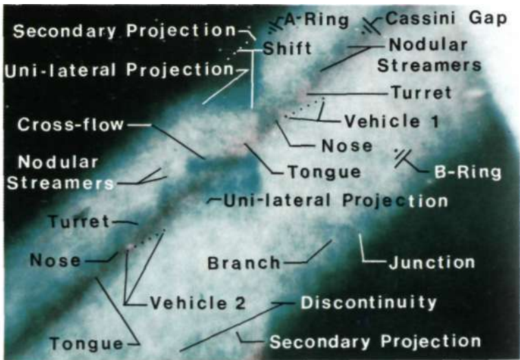
Plate 20: Apparent ring shift and band discontinuity in relation to two electromagnetic vehicles in the Cassini gap.
