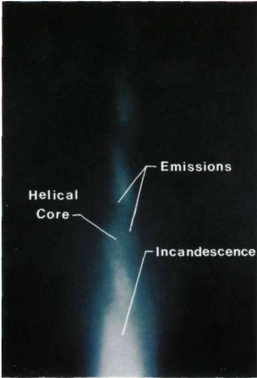
(b) Region (2), plate 23
